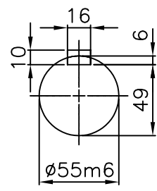
VIEW "A" SCALE 4/1
