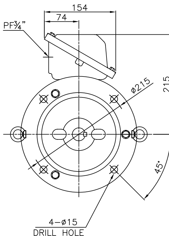
VIEW "A"
